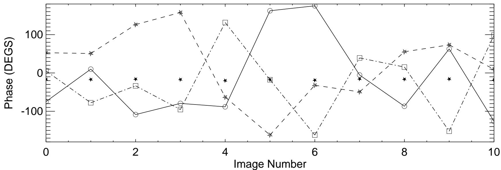
MIRC Closure Phases
