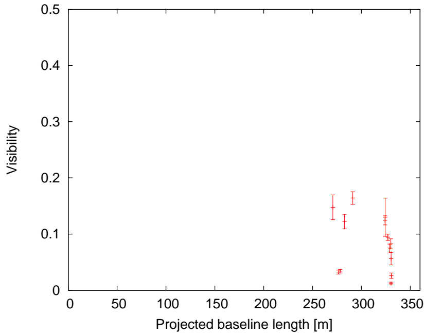
MWC340, CHARA/CLASSIC data (2010Jul20, 2010Jul21)
